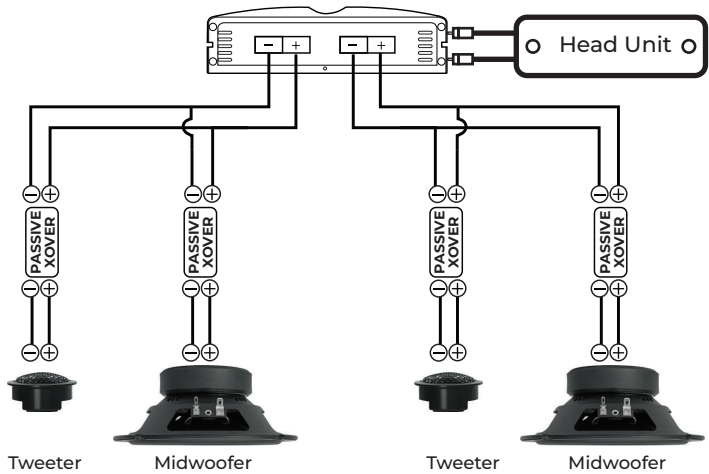
2 Channel Amplifier
