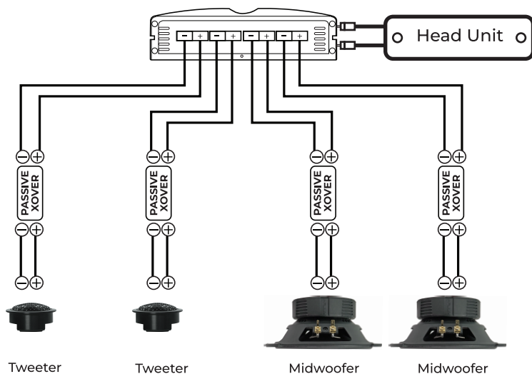
4 Channel Amplifier
