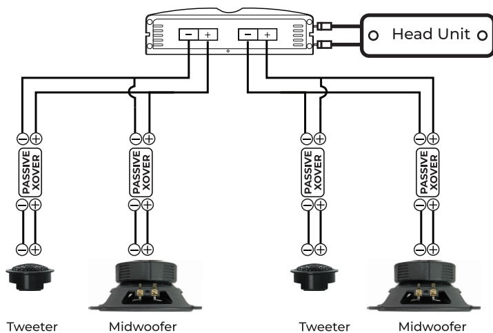
2 Channel Amplifier
